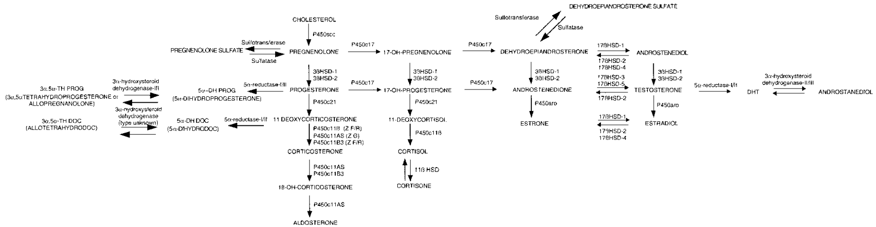
Fig. 1. Pathway for the biosynthesis of neurosteroids in the nervous system. The names for each enzyme are shown by each reaction. P450sc, mitochondrial cholesterol side-chain cleavage enzyme, mediates 20 \alpha hydroxylation, 22 hydroxylation, and scission of the c20–22 bond; 3 \beta HSD, a non P450 enzyme(s) bound to the endoplasmic reticulum mediates both 3 \beta hydroxysteroid dehydrogenase and \Delta 5– \Delta 4 isomerase activities; P450c11 \beta , mitochondrial 11 hydroxylase, mediates 11 hydroxylation; P450c11AS, mitochondrial aldosterone synthase, mediates c11,18 hydroxylation and 18 oxidation; Z F/R and Z G refer to the adrenal zona fasciculata/reticularis, or zona glomerulosa, that express the particular P450c11 gene; 17 \beta HSD (also called 17 ketosteroid reductase, or 17 KSR), mediates c17 \beta reduction or c17 oxidation. Virtually all these enzymes have been identified in the brains of various species, with the notable exception of P450c21. 21 hydroxylating activity has been demonstrated, but may not be due to P450c21. Synthesis of steroid sulfates mediated by sulfotransferase and sulfatase are also shown.
